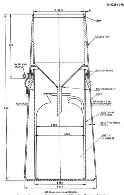
IS 5225 : 1992 All dimensions in millimeters. FIG. 1 Bala JI HydroMet Non-Recording ( 200 cm 2 ), GENERAL ASSEMBLY
